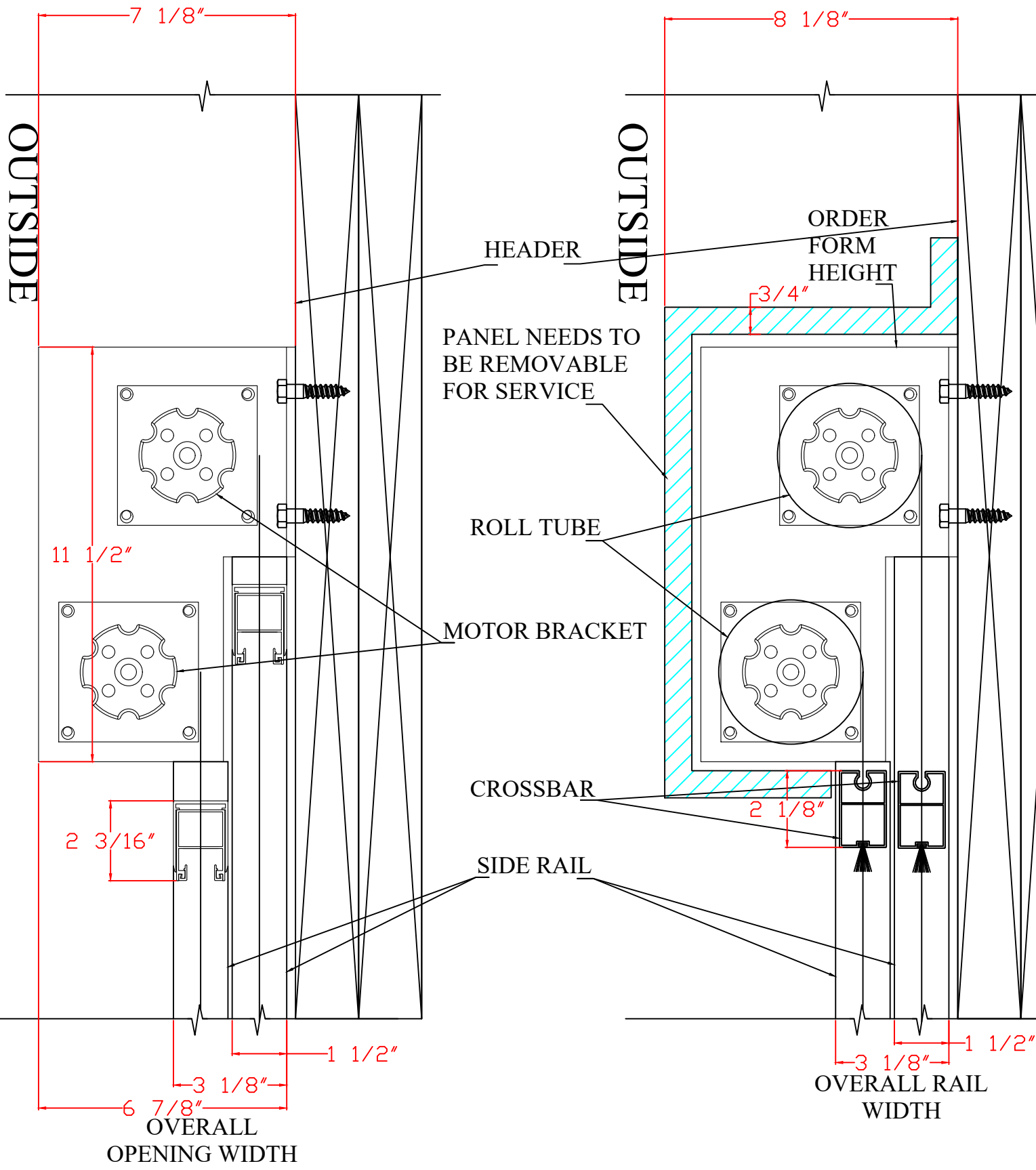
CROSS SECTION OF THE DUAL ROLL TUBE OUTSIDE ABOVE HEADER INSTALL
