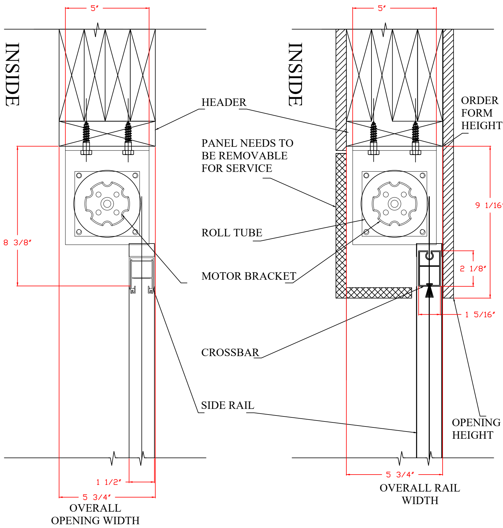
CROSS SECTION OF THE SINGLE NO HOUSING ROLL TUBE UNDER HEADER INSTALL
