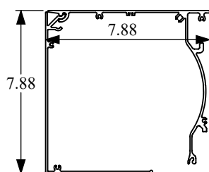
Series 3 Housing
