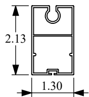
Crossbar
